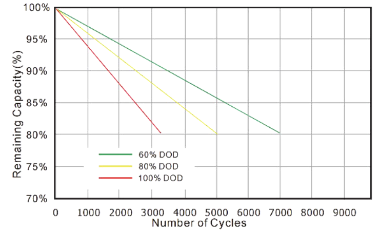
Different Discharge Depth Life Curves & 40°C, 0.5C
