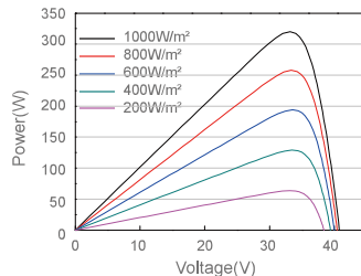
Power-Voltage Curve JAM60S12-320/PR
